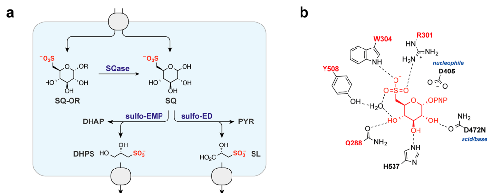
Figure 1. Role of sulfoquinovosidases (SQases) in allowing sulfoglycolytic utilization of sulfoquinovose glycosides. (a) Sulfoglycolysis pathways in bacteria highlighting proposed role of sulfoquinovosidases. (b) Cartoon of active-site residues involved in binding PNPSQ from the X-ray structure of E. coli YihQ D472N.
